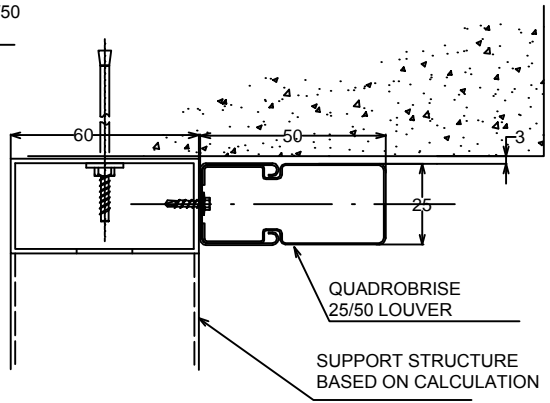
Upper Detail
