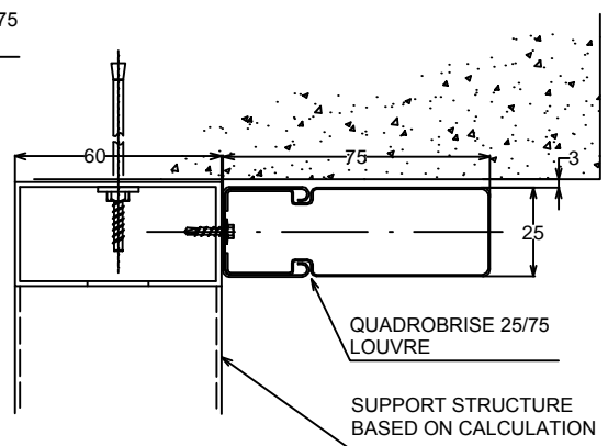
Upper Detail
