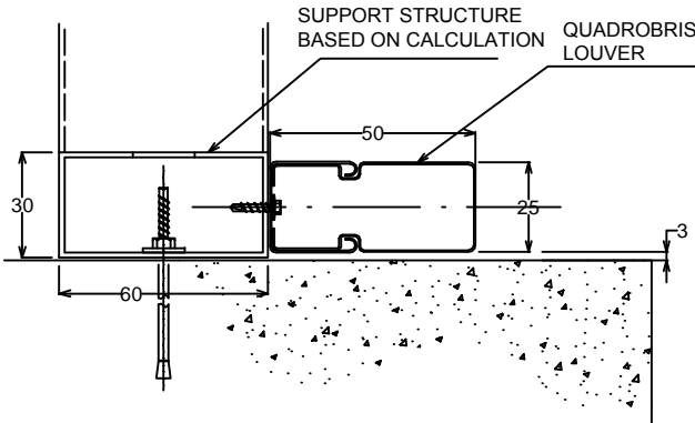
Lower Detail
