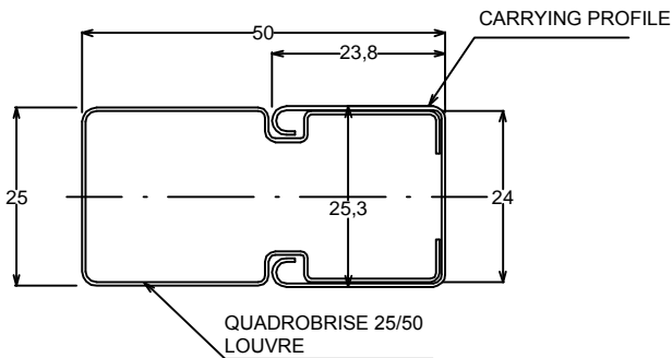
CUT B - B
