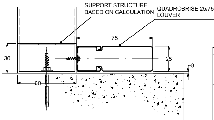
Lower Detail
