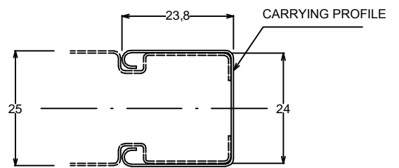
Quadrobrise 25/50 Carrying Profile
