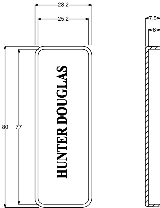
QUADROBRISE 25/75 COVER MATERIAL : ALUMINIUM
