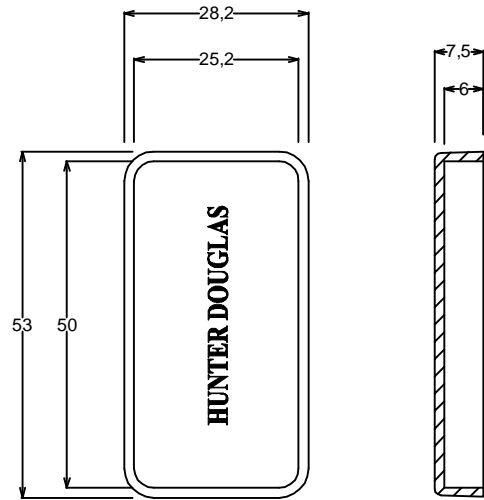
QUADROBRISE 25/50 COVER MATERIAL : ALUMINIUM
